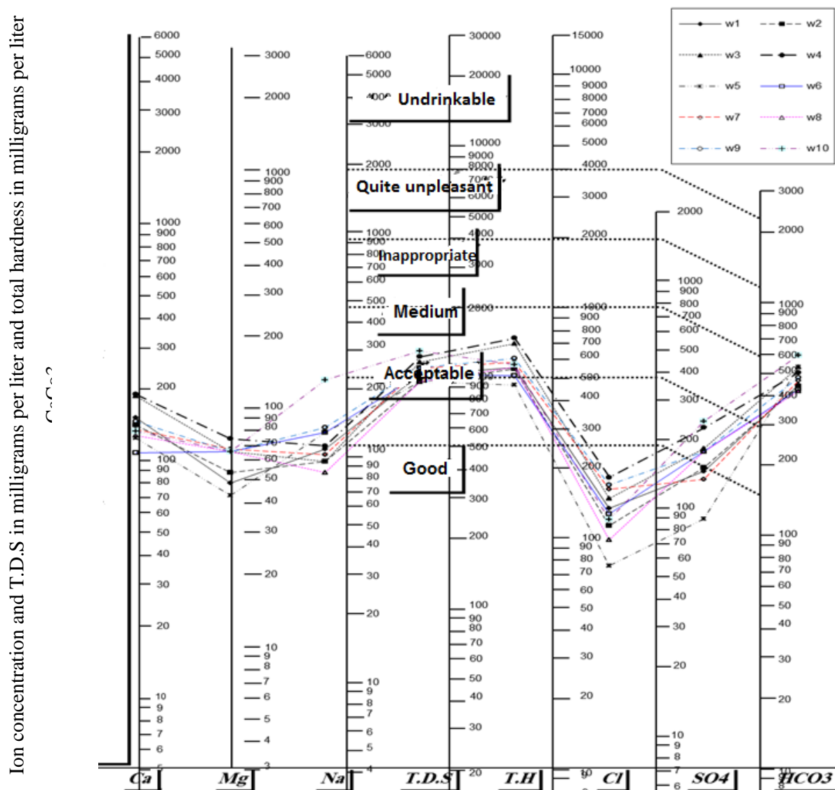
Fig2 . Schuler diagram for classification of drinking water quality
