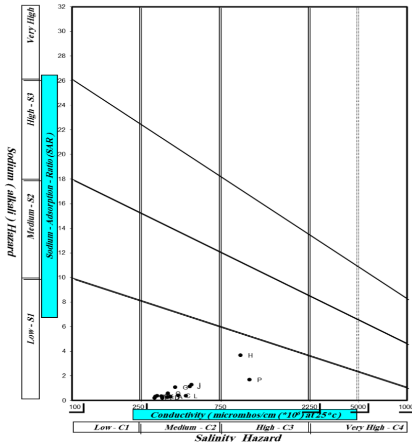
Fig3. Wilcox diagram for classification of water quality for agriculture - irrigation
