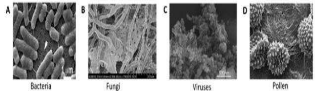
(b) Images of different types of microbial bioaerosol captured from electron microscope
