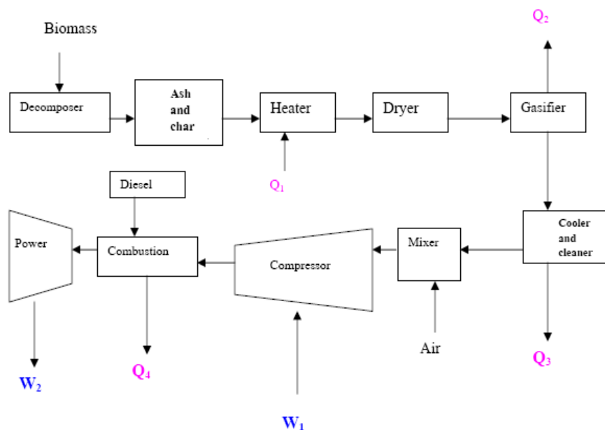
Fig7. Advanced biomass power with diesel engine (Omer, 2006)
