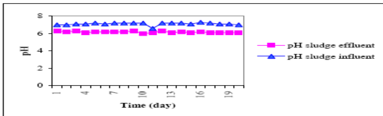
Fig6. Potential of hydrogen (pH) sludge before and after treatment in the digester (Omer, 2006)
