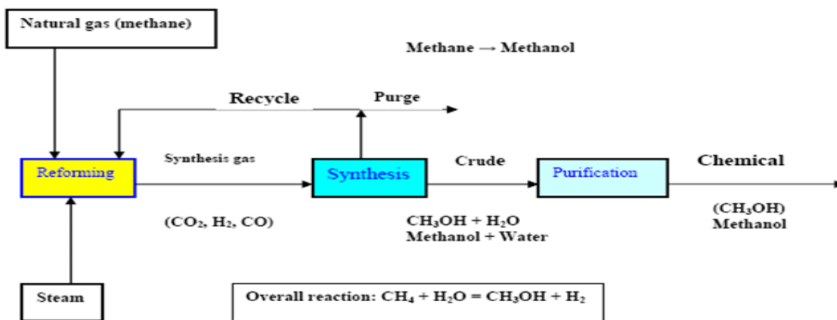
Fig2. Schematic diagram shows methanol production (Omer, 2006).
