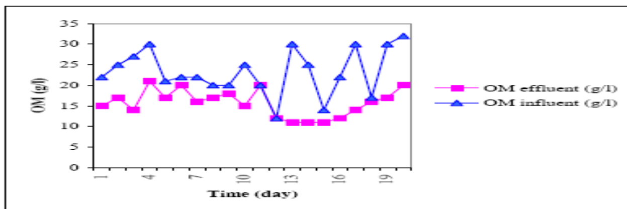
Fig5. Organic matters before and after treatment in digester (Omer, 2006).
