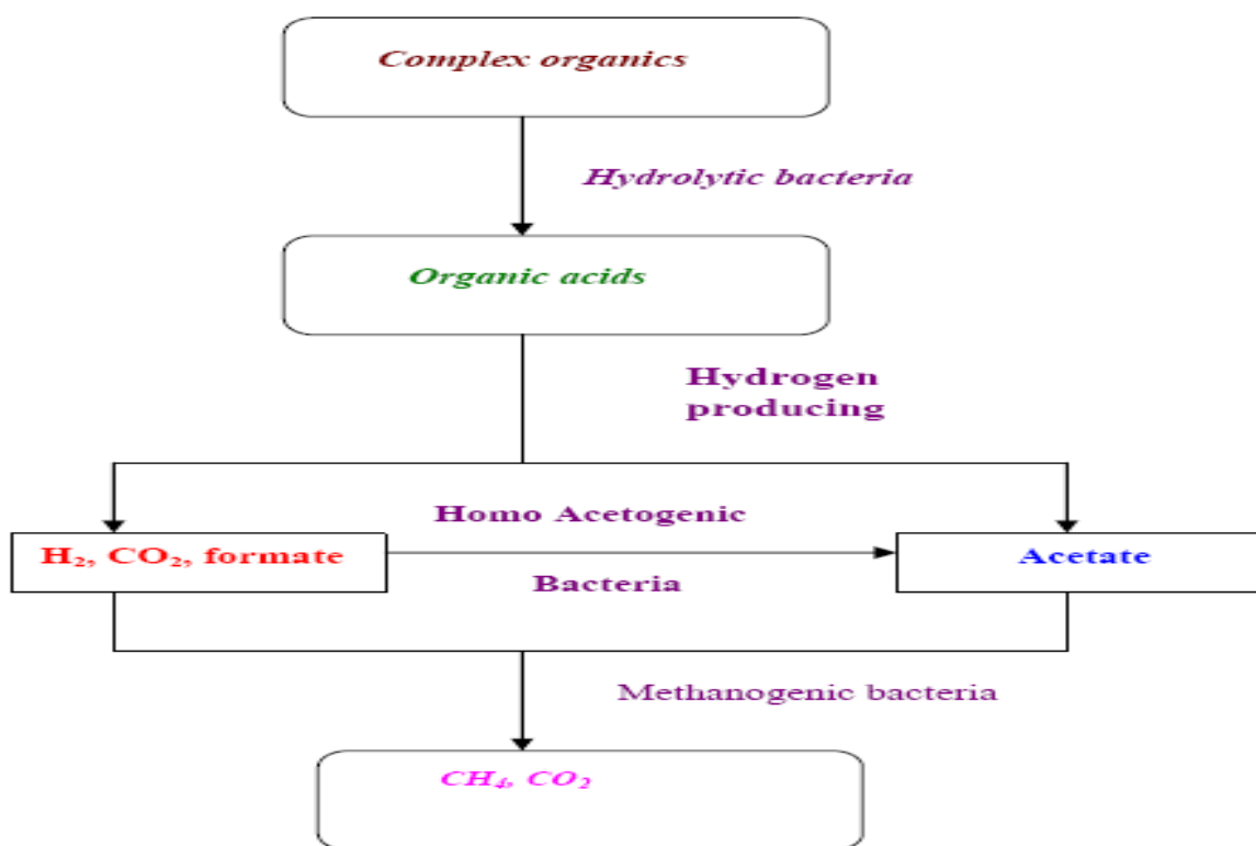
Fig3. Biogas production process (Omer, 2003).
